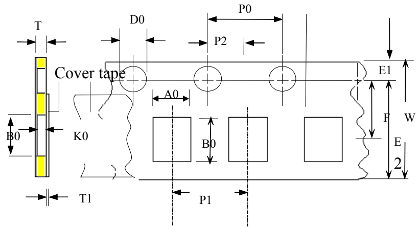
Paper Tape Component Dimensions
